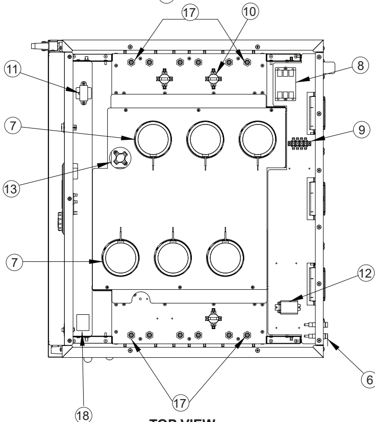
TOP VIEW WITHOUT COVER
